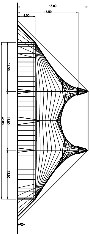
LATERAL VIEW
