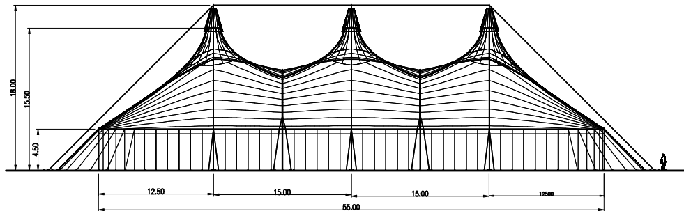
LATERAL VIEW
